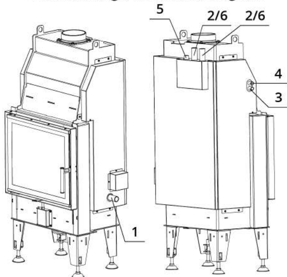
Heat exchanger connection diagram
